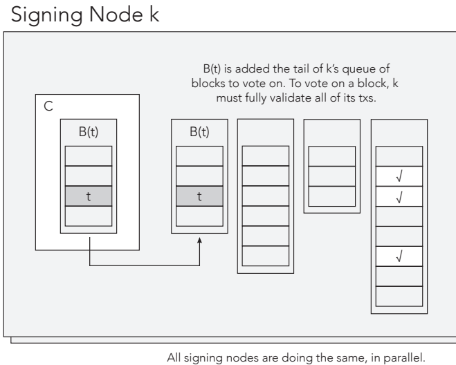
Figure 12: Life of a Transaction, Part 2/2
